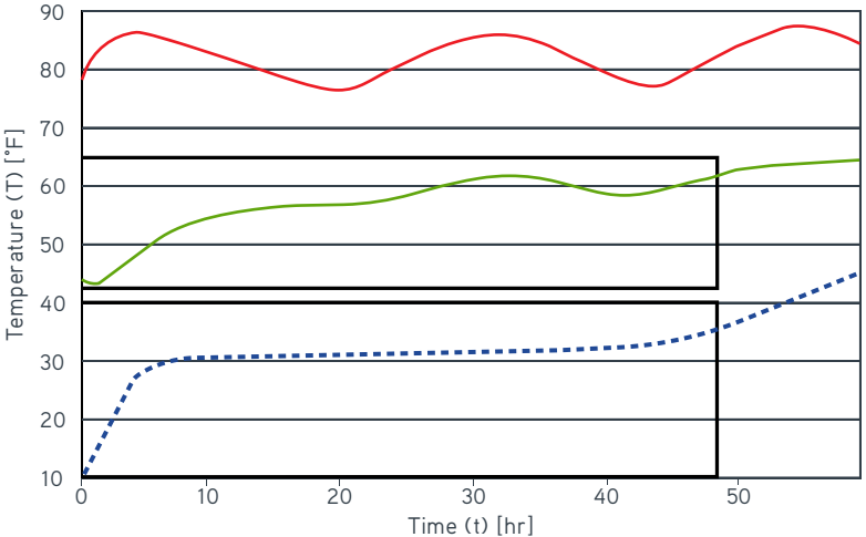
Meal Kit Delivery – ISTA 7E Hot Profile
